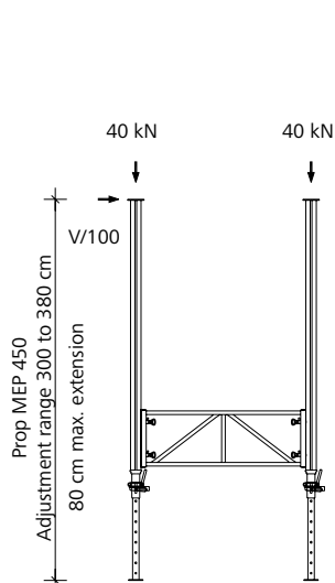
Fig. 5.1 Freestanding. Horizontal load is transferred through the tower.
