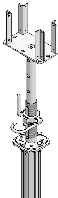
Fig. 10.3 With forked prop head MEP
