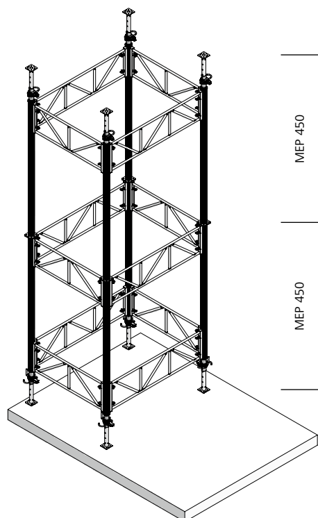
Fig. 33.3 Adjustment range 6,00 to 9,00 m
