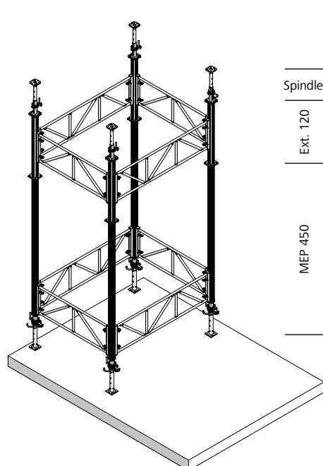
Fig. 33.1 Adjustment range 4,48 to 6,50 m
