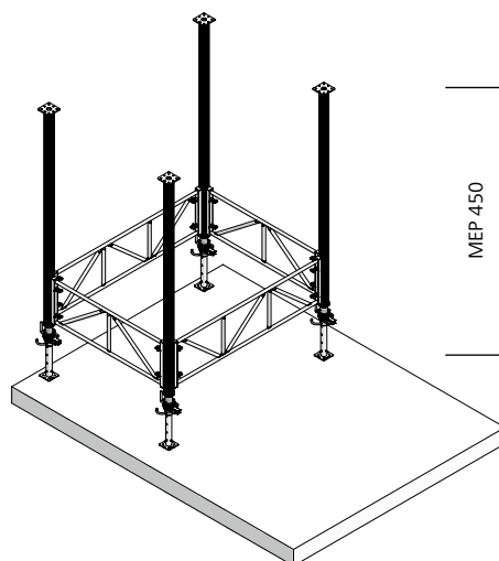
Fig. 32.3 Adjustment range 3,00 to 4,50 m
