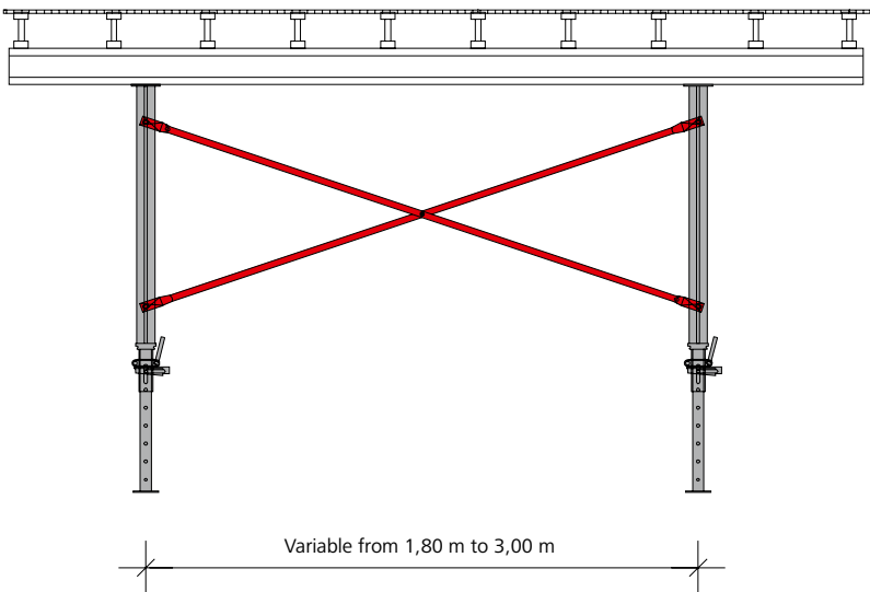
Fig. 11.2 Use with table form
