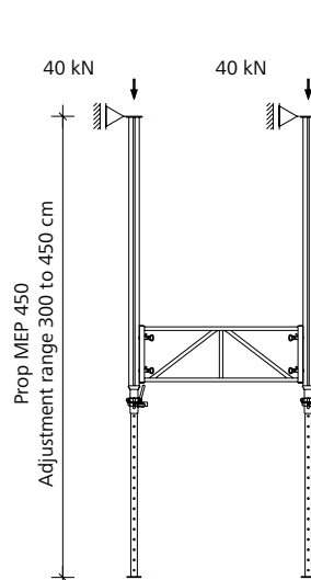
Fig. 5.2 System attached at top
