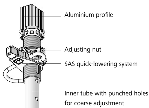
Fig. 6.3 SAS quick-lowering system
