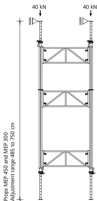
Fig. 5.4 System attached at top
