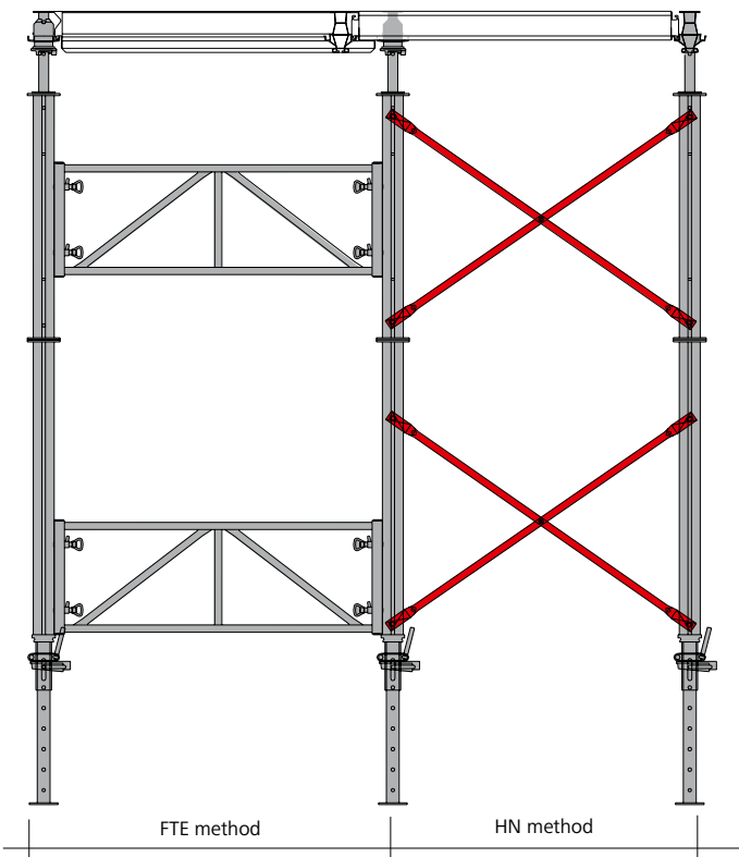
Fig. 11.1 Example: MEP shoring tower with MevaDec for rooms higher than 4,90 m
