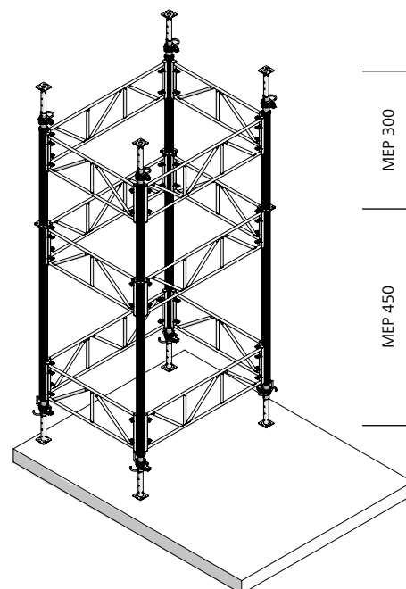
Fig. 33.2 Adjustment range 4,85 to 7,50 m
