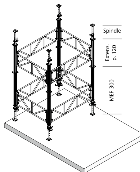
Fig. 32.2 Adjustment range 3,33 to 5,00 m
