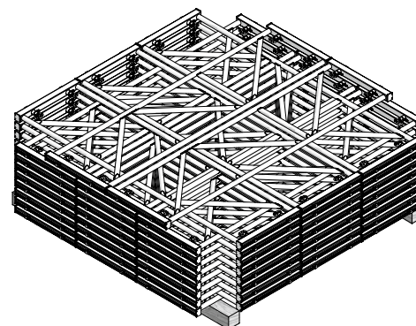
Fig. 35.4 Bundle of frames 220 MEP
