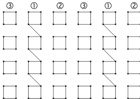
Fig. 18.3 Diagonal cross-braces for towers up to 6 m high
