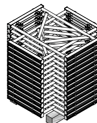
Fig. 35.2 Bundle of frames 110 MEP
