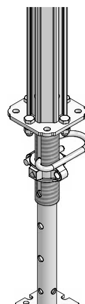
Fig. 10.4 Spindle used as foot spindle
