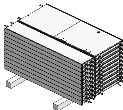
Fig. 35.6 Scaffold platforms piled on square timber
