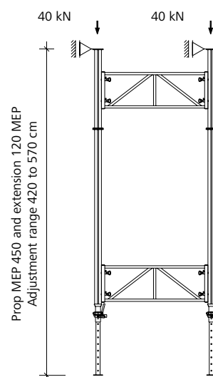
Fig. 5.2 System attached at top
