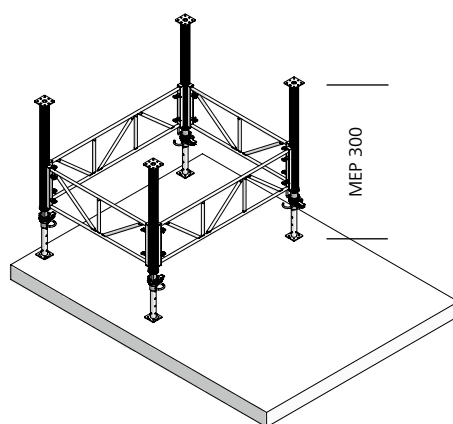
Fig. 32.1 Adjustment range 1,85 to 3,00 m
