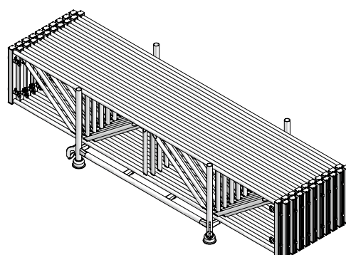
Fig. 35.5 Frames 330 MEP in piling rack
