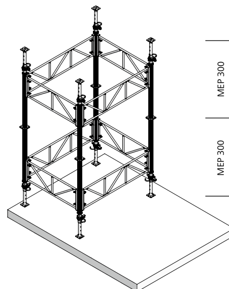
Fig. 32.4 Adjustment range 3,70 to 6,00 m
