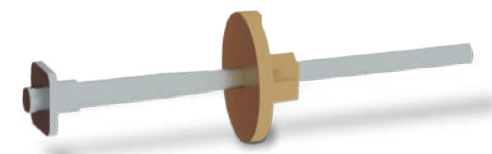
EF Tension Screw to form external corners
