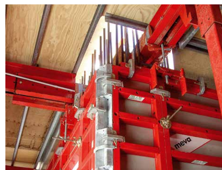
The wall formwork panels are suspended, can be moved back manually, and allow the formwork to be opened quickly and easily.
