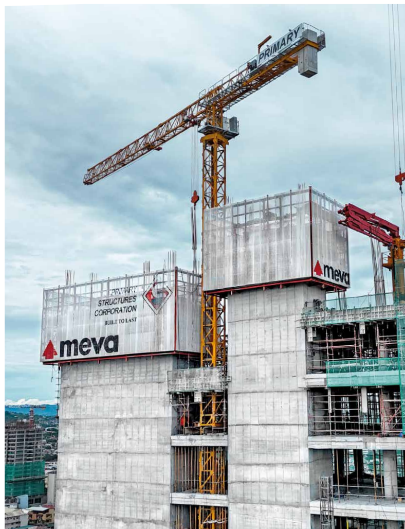
The central location in Cebu City made logistics difficult. Right: The cooperation between Primary Structures Corporation and MEVA went smoothly. Below: The enclosed MAC climbing systems protected the workers from wind and weather.
