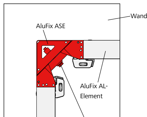
Abb. 29.4 – Detail A
